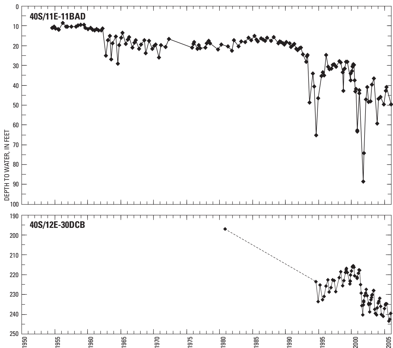
Figure 35. Water-level fluctuations in wells 40S/11E-11BAD in the southern Poe Valley and well 40S/12E-30DCB north of Malin, Oregon.
